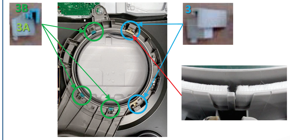
Position of Bearing and Seal join
